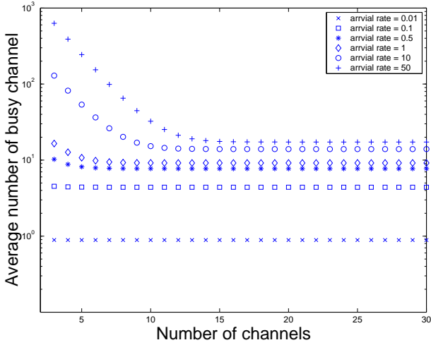
Fig. 6. Average Number of Busy Channels vs. Number of Channels with Different Client Workload
